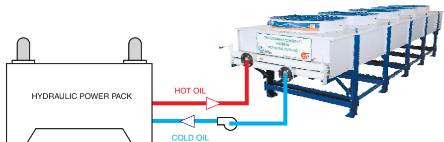
WITHOUT HEAT EXCHANGER
