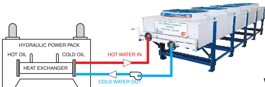
WITH HEAT EXCHANGER
